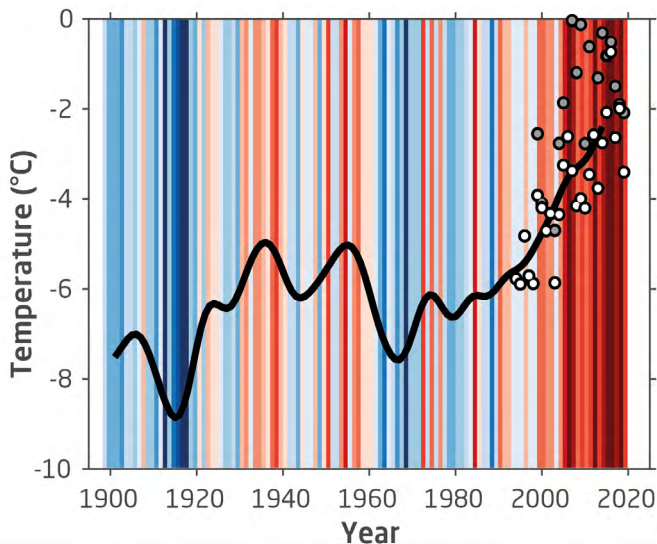
Figure 1: Temperature record of Svalbard. Black curve: long-term record at Svalbard Airport in Longyearbyen (low pass filtered data of the Norwegian Meteorological Institute 21 ). Surface air temperature (white dots) and soil temperature at 59 cm depth (grey dots) recorded at the AWIPEV research base. Warming Stripes for Svalbard (source: Ed Hawkins CC BY 4.0).
